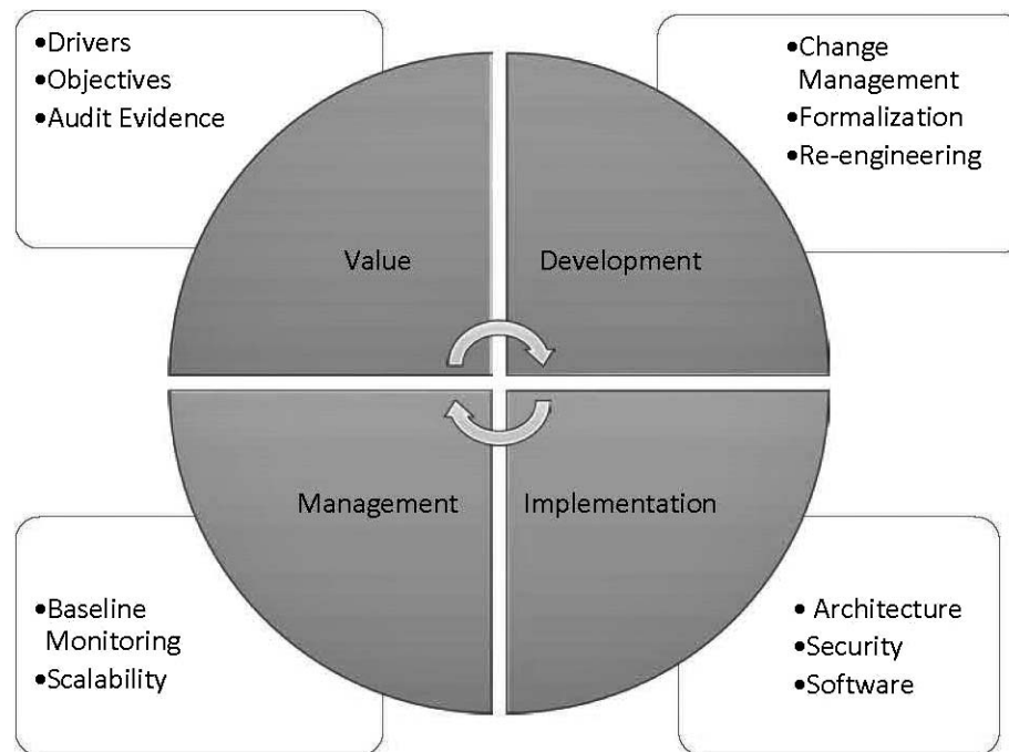
FIGURE 2 Audit Automation
